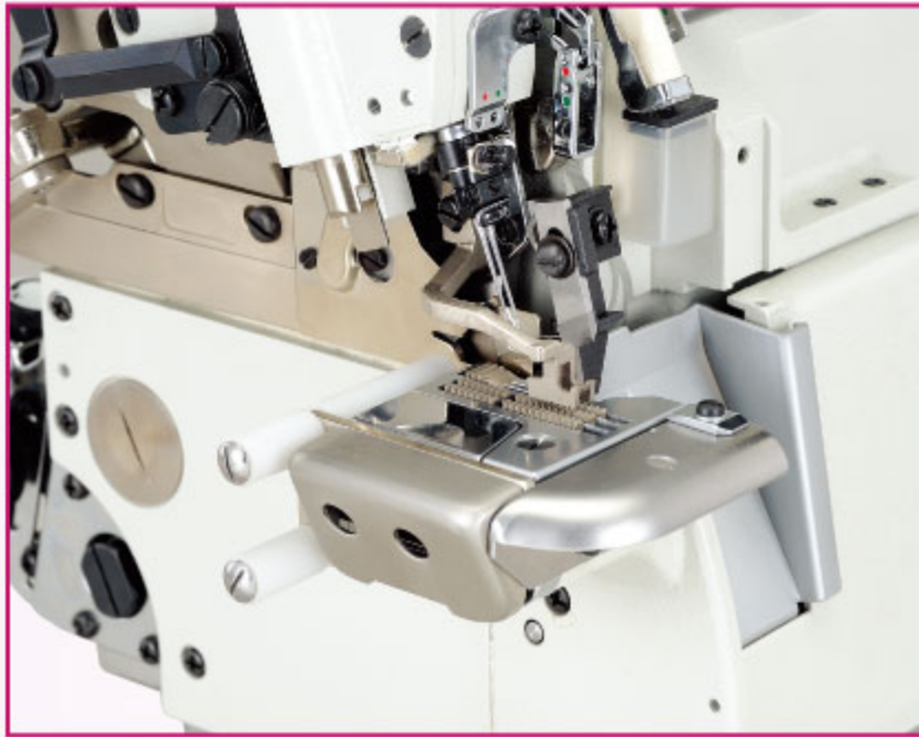
SS038:側吸風式自動切線刀(垂直吸風式) Side suction type thread trimmer (vertical type).
