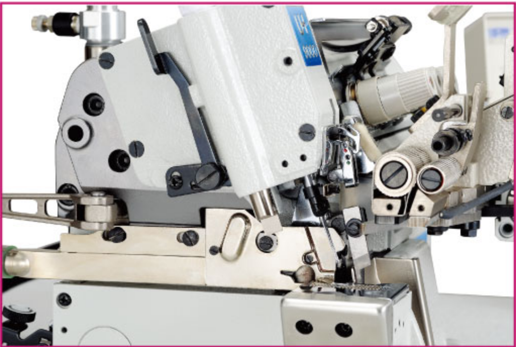
適用於有安裝吸入式線頭切斷裝置的包縫車 Suitable for overlock with chain cutter and lint collector.
