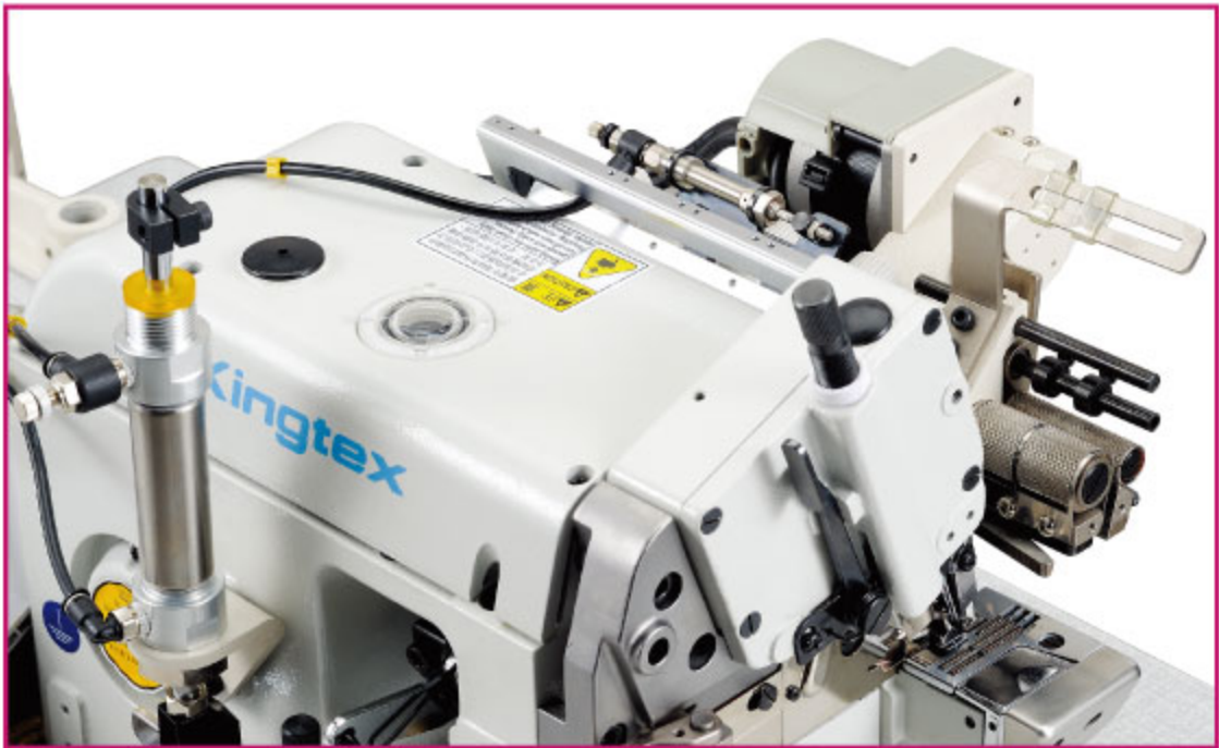
縫畢時可將車針的縫線放鬆便於切斷 Release the thread for cutting thread easily after sewing.
