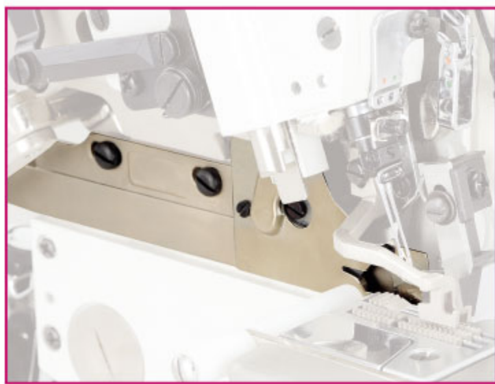
SS038:側吸風式自動切線刀(垂直吸風式) Side suction type thread trimmer (vertical type).
