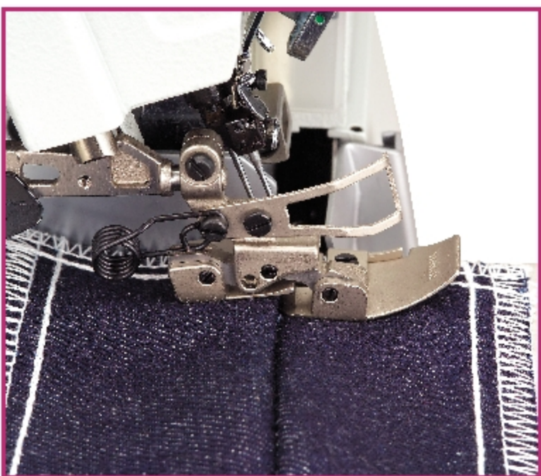
浮動壓腳 Tractor presser foot
