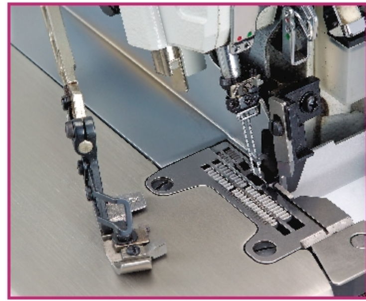
包縫頭車縫 (4線) Backlatching device (4-Thread)
