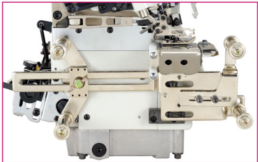
筒型衣物撐開滾輪組 (TR012) FABRIC TENSION CONTROLLING DEVICE 可依衣物長短配合選用。 TR012 適用範圍 500 ~ 800 mm。 (TENSION ROLLER) Can be used for different lengths of garments Suitable length: 500 ~ 800 m.m.
